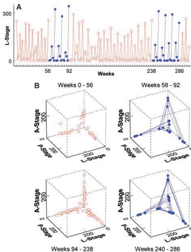
Fig. 4. A 304-week data time series obtained from one replicate of the Tribolium experiment (3). Parameter values are b = 10.67 , \mu_l = 0.1955 , \mu_a = 0.96 , c_{el} = 0.01647 , c_{ea} = 0.01313 , and c_{pa} = 0.35 . (A) Selected temporal episodes that resemble the lattice model 6-cycle shown in Fig. 3B are colored in blue. The remaining data points, colored in red, resemble the chaotic time series. (B) The selected temporal episodes in (A) are shown in phase space (on the order of 10^7 lattice points). Compare the blue 6-pattern episodes to the 6-cycle lattice attractor in Fig. 3B.
