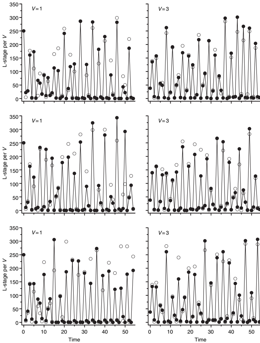
Figure 1 Time series of L -stage densities for the six experimental populations. Closed circles are the observed densities and open circles are the one-step predictions for the deterministic model (1) with parameter values b = 10.67 , c_{el} = 0.01647 , c_{ca} = 0.01313 , c_{pa} = 0.35 , \mu_1 = 0.1955 and \mu_a = 0.96 . On the left are the populations cultured in 20 g of media ( V = 1 ); on the right are the populations cultured in 60 g of media ( V = 3 ).
